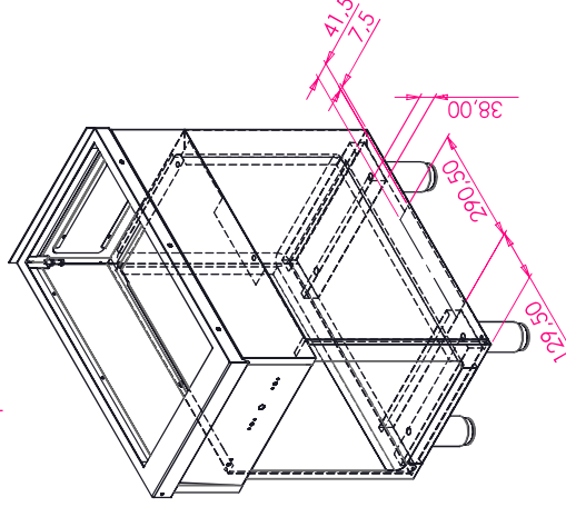
Position Kabeleinführung/ position cable intake
