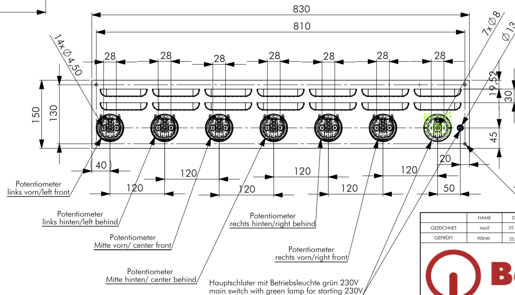
Schalterblende (optional lieferbar) switch panel - optional available
